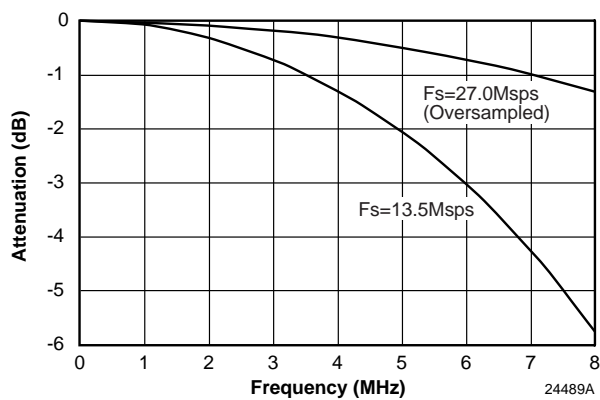
Figure 12. \sin(x)/x Response
