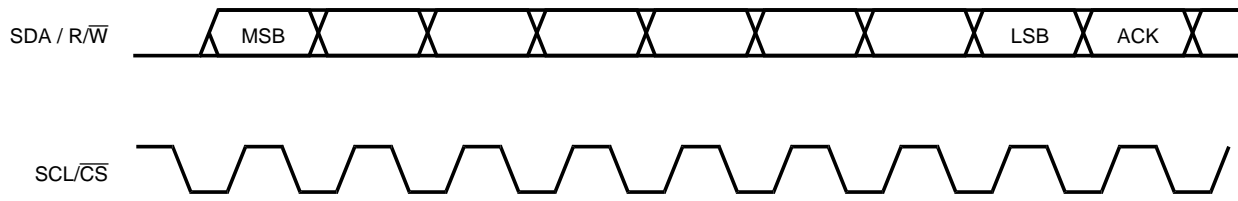
Figure 16. Serial Interface – Typical Byte Transfer
